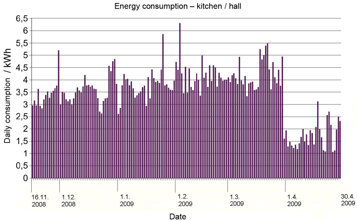
Pic. 4.2: Energy consumption of group 2 (kitchen / hall)
