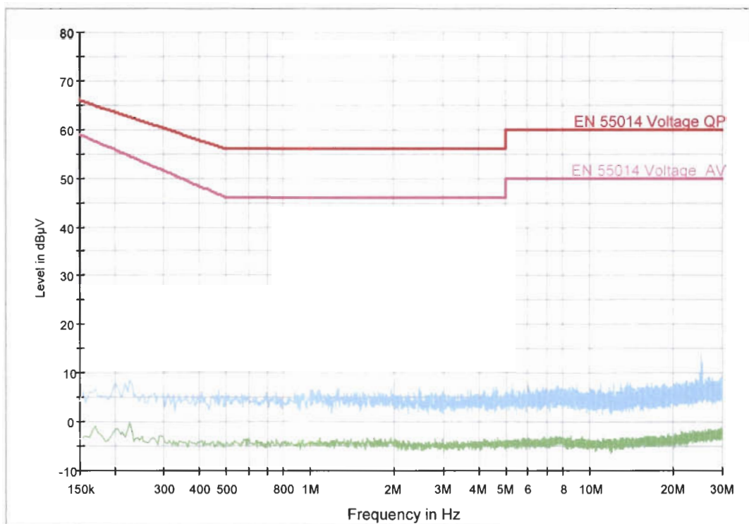
EN55014Voltage
