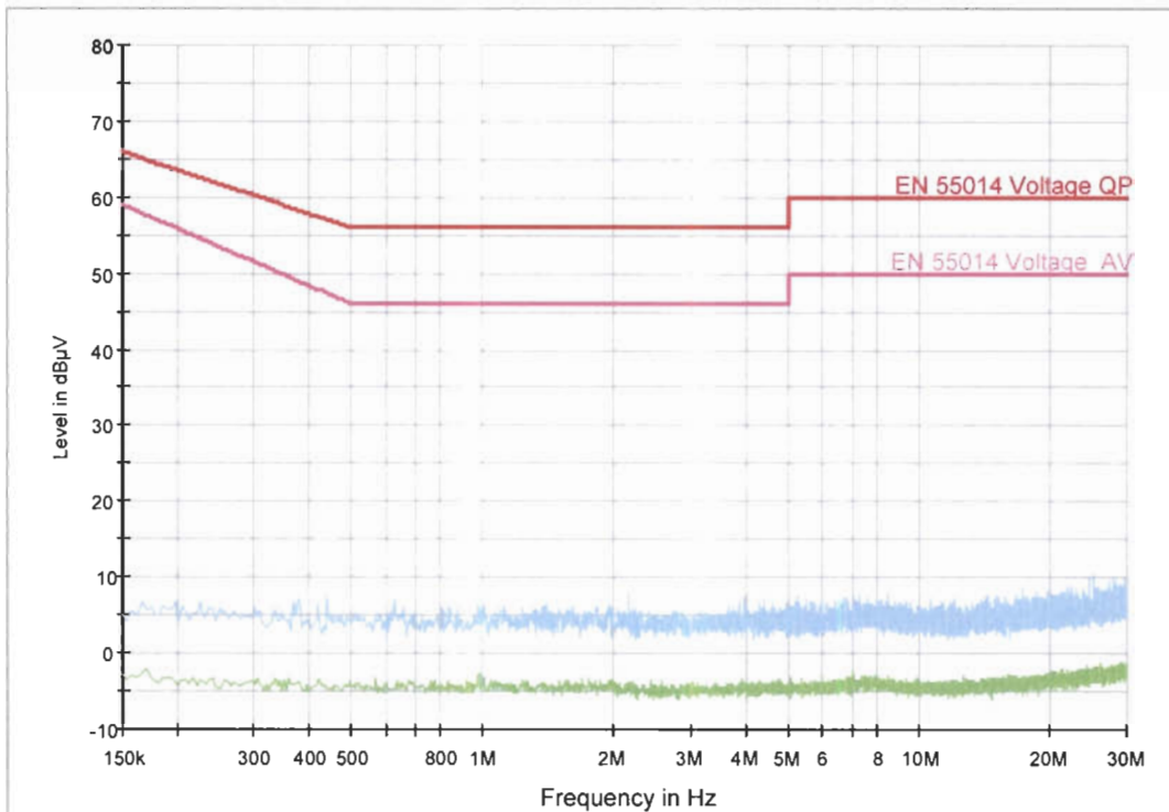
EN55014Voltage
